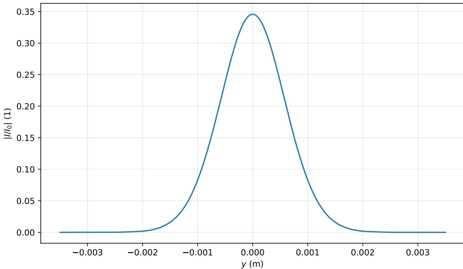
Intensity profile I(x=0, y, z=3.184)/I_0 , P_{in}=0.2P_{cr} , artificial time
